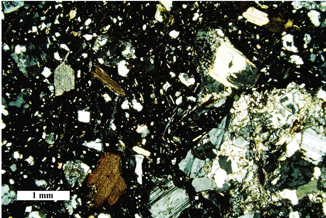
Figure 6.6. Polygranular quartz + K-feldspar (microcline) + mafic igneous rock fragments (right of center) in sample JMHO33 (cross-polarized light). The feldspar displays fine-grained sericite alteration. Other aplastic inclusions include blocky, golden brown biotite crystals (left of center) and blocky microcline (twinned; bottom center).
