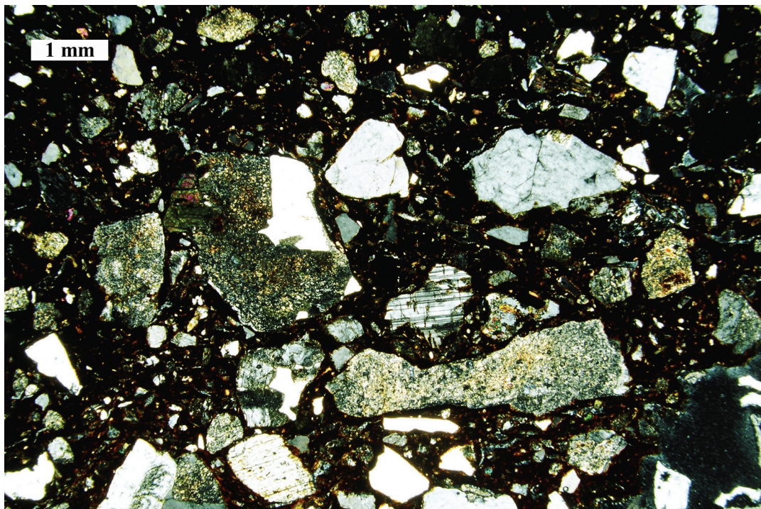
Figure 6.7. Highly-altered quartz + feldspar rock fragments (left of center) and feldspar mineral fragments (bottom center) in sample JMH048 (cross-polarized light). The feldspar in the rock and mineral fragments displays fine-grained sericite alteration. Also note the unaltered blocky plagioclase fragment (polysynthetic twinning; center).
